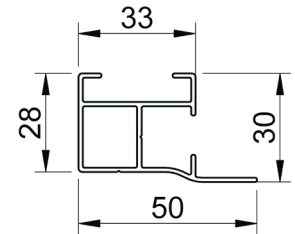
en option: glissière fabric cover 28mm P x 50mm L
