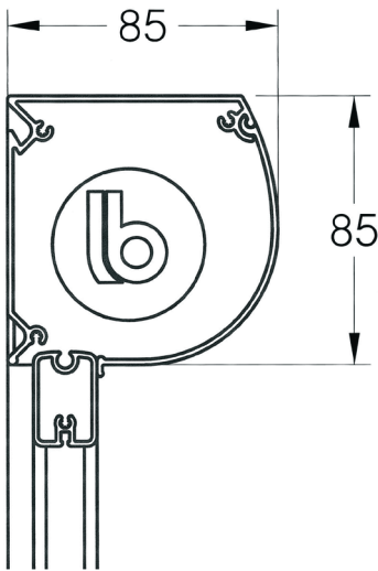
boîtier 85mm x 85mm barre de charge 20mm P x 30mm H
