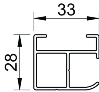
glissière standard 28mm P x 33mm L
