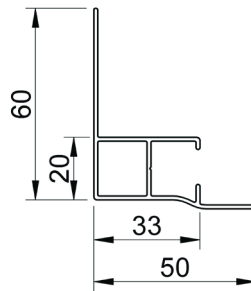
en option: glissière side fix fabric cover 60mm P x 50mm L
